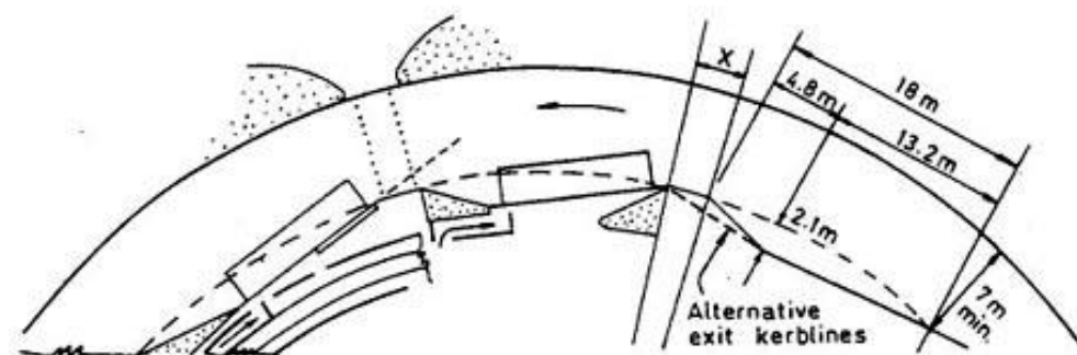
(F) CURVE-INTERNAL KERB, SMALL RADIUS
