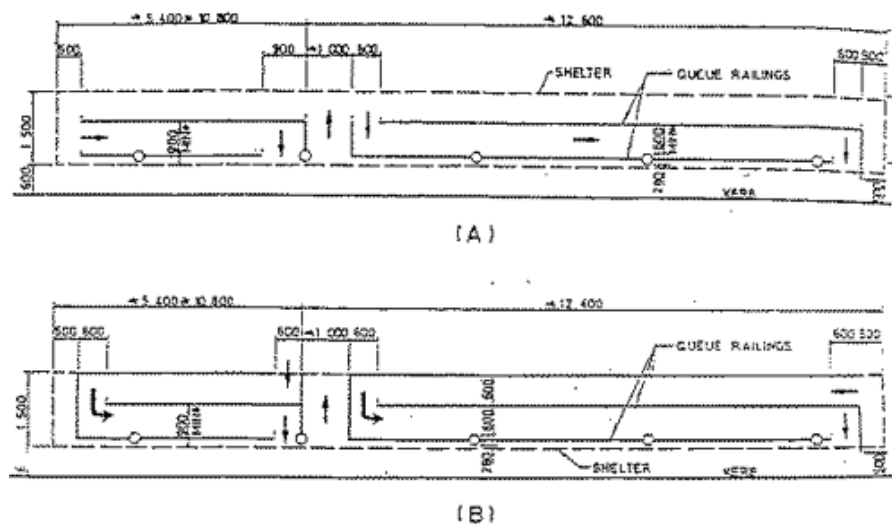
DIAGRAM 2.6.3.5: SETTING OUT DETAILS FOR STANDARD QUEUE RAILING AT ADJACENT STOPS SCALE 1:200
