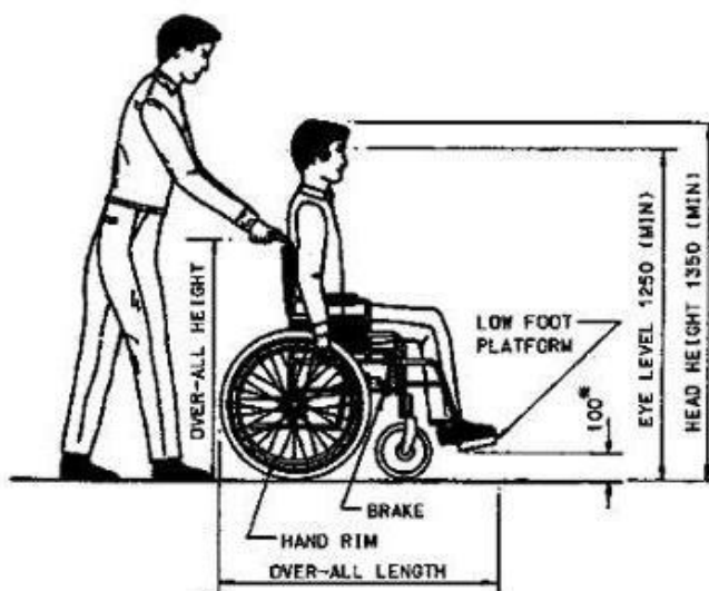
DIAGRAM 8.2.3.1 : DIMENSIONS OF WHEELCHAIRS
