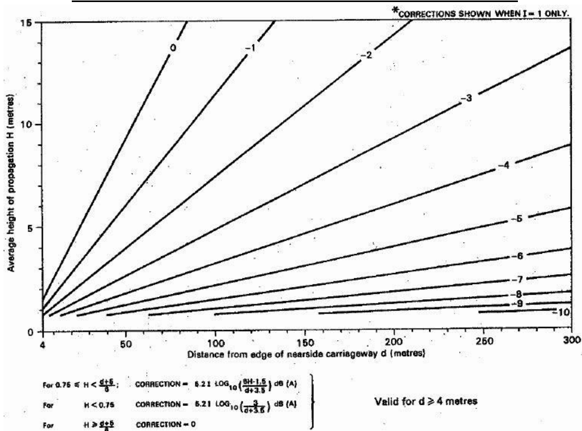
DIAGRAM 7.4.2.5 : CORRECTION FOR GROUND ABSORPTION
