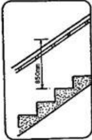
HANDRAILS ABOVE STEPS NEED TO BE AT A LOWER HEIGHT THAN IN RESPECT OF LEVEL SURFACES.
