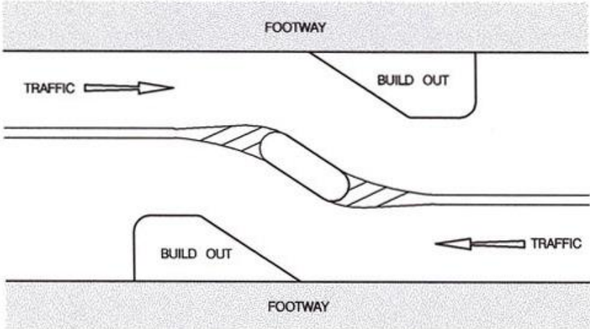
TWO-WAY WORKING CHICANE
