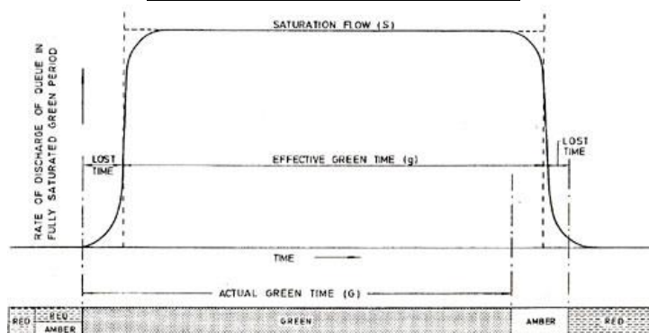
DIAGRAM 2.4.1.1: VARIATION WITH TIME OF DISCHARGE RATE OF QUEUE IN A FULLY SATURATED GREEN PERIOD
