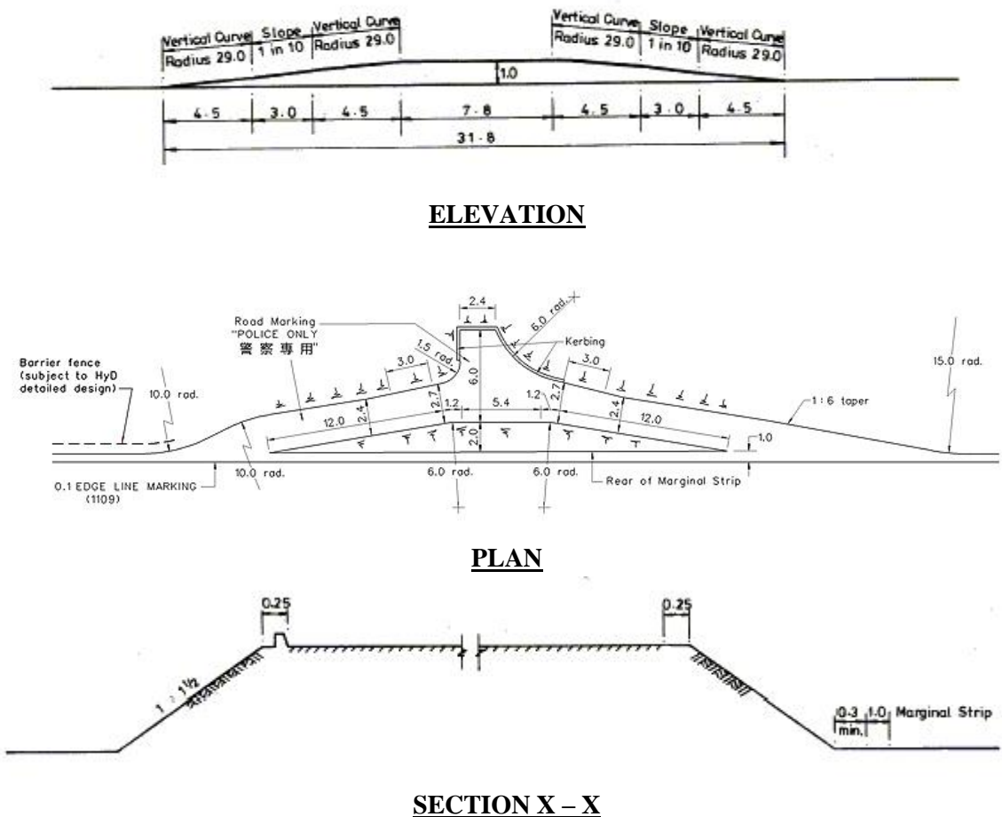
DIAGRAM 3.4.10.1 : POLICE OBSERVATION PLATFORM TYPICAL LAYOUT, ELEVATION AND SECTION
