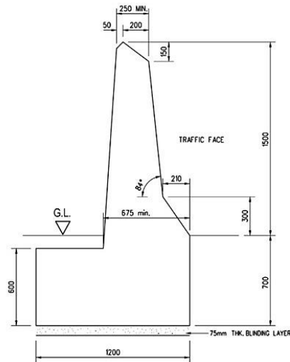
TYPICAL DETAILS OF L4 HIGH CONTAINMENT BARRIER
