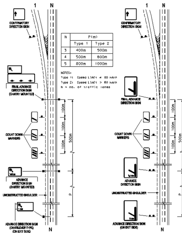
(a) Layout for Gantry Signs
