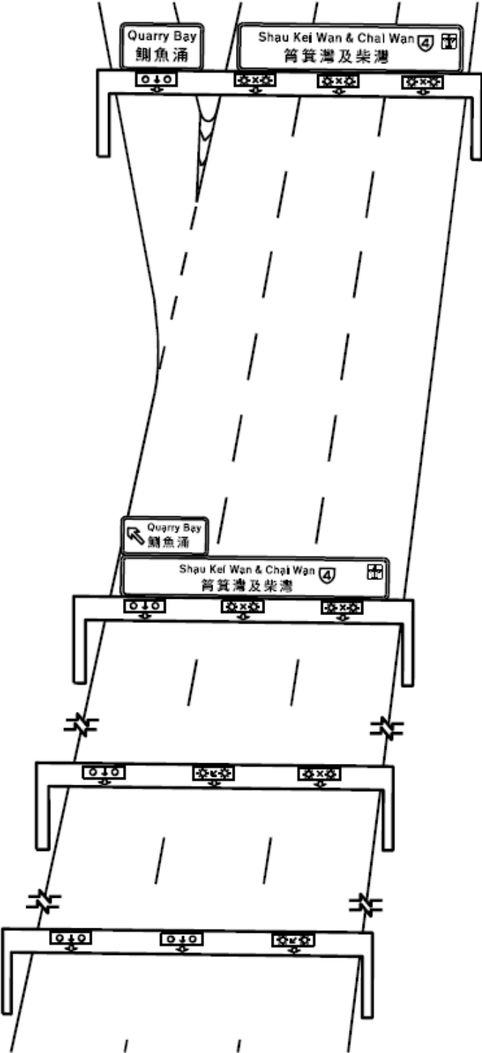
FIGURE 5.5: CARRIAGEWAY CLOSURE
